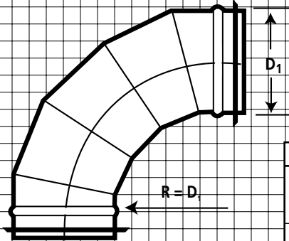
90° 5-PC. ELBOW E90T
