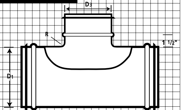
PRESSED TEE PTT
